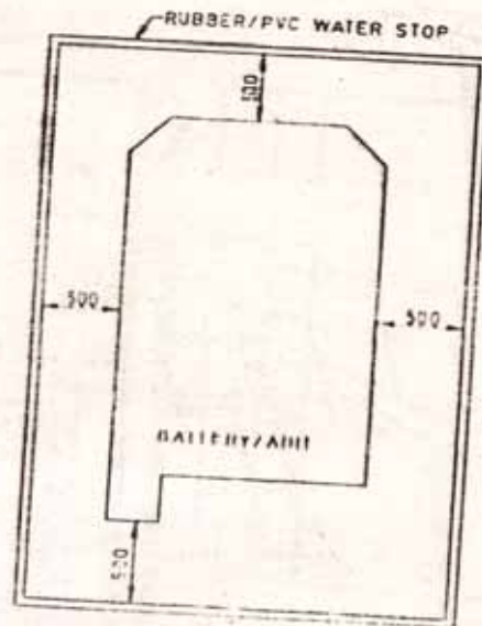
FIG. A RUBBER/PVC WATERSTOP AROUND GALLERY/ADIT AT CONTRACTION JOINTS
