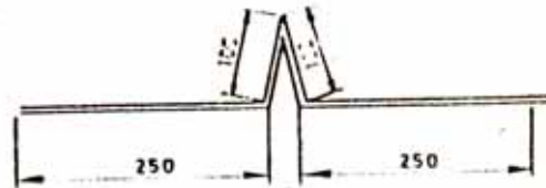
1B DETAILS OF M-SHAPE METAL WATER STOP
