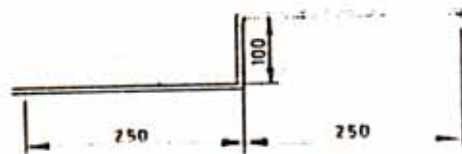
1A DETAILS OF Z-SHAPE METAL WATER STOP
