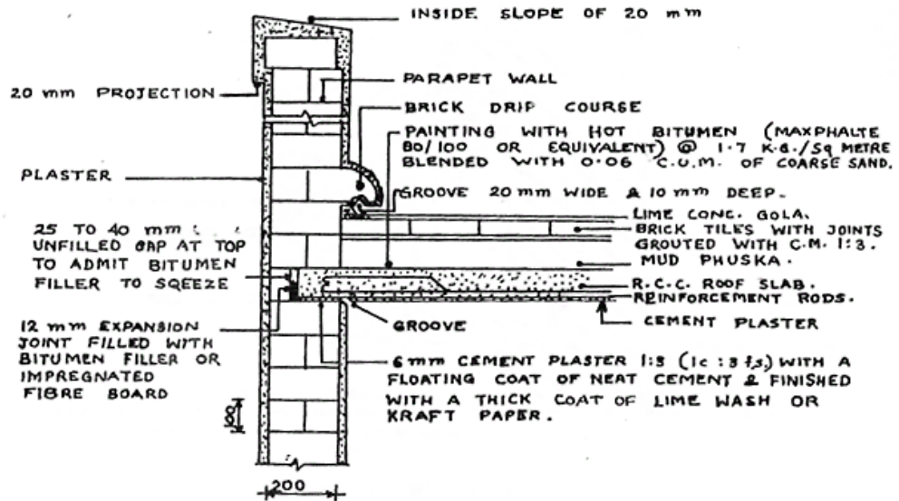
SECTION AT RIDGE
