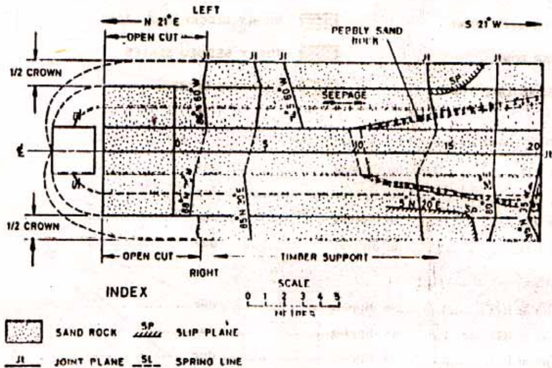
TYPICAL EXAMPLE OF A THREE-DIMENSIONAL LOG OF EXPLORATORY DRIFT
