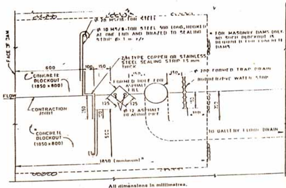
FIG. C SECTIONAL PLAN AT CONTRACTION JOINT (DOWEL BARS BETWEEN PRECAST MASSURE FACE OF THE BLOCKOUT NOT SHOWN (See Clause 7.3) )
