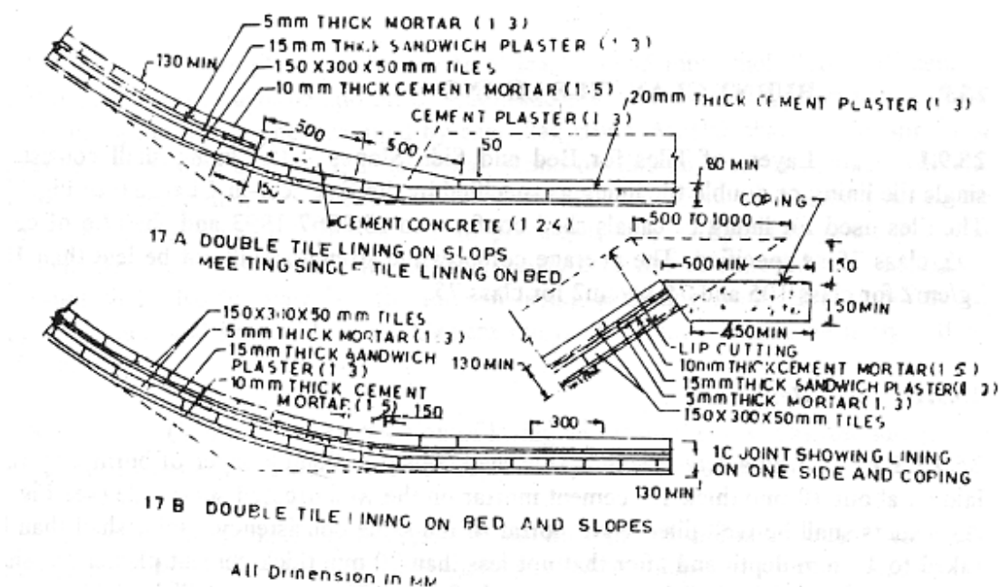
Fig. 17 Typical Sketch Of Canal Lining With Burnt Clay Tiles
