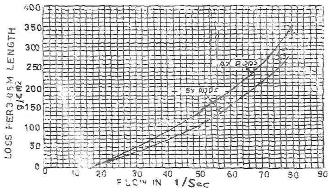
8B : HEAD LOSS PER 3.05 SECTION IN AX AND BX RODS
