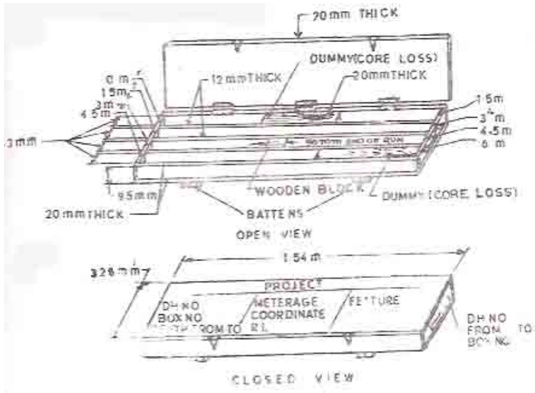
Fig. Typical Details of Core Box For 54.7 MM Dia Core
