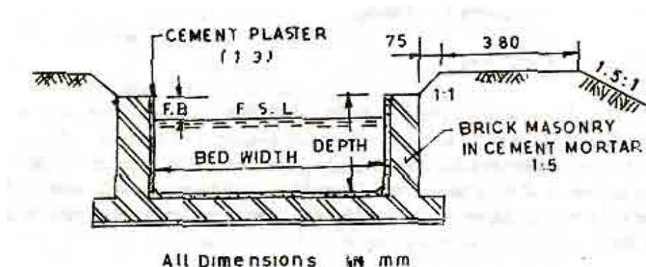
Fig. 19 Typical Brick Masonry Section
