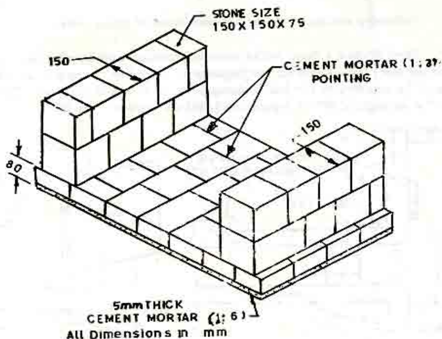
Fig. 23 Stone Masonry Lining
