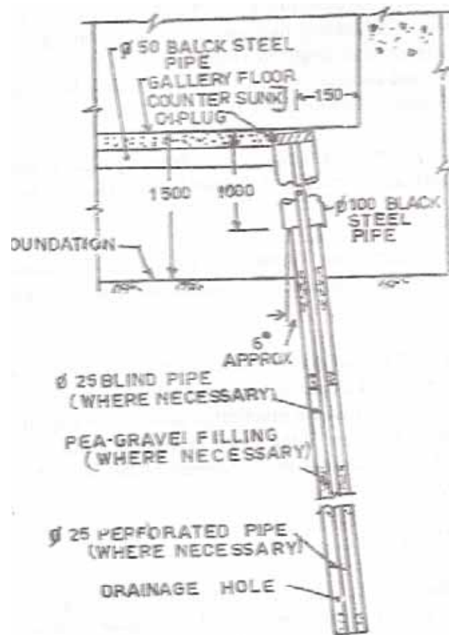
Fig. 6 B. Foundation Drainage Pipe (In Soft Foundation) (All Dimensions In MM)
