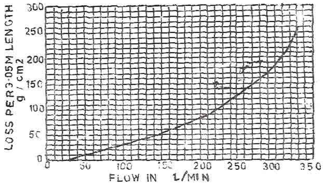
8A : HEAD LOSS PER 3.05 M. LENGTH IN 32 MM PIPE
