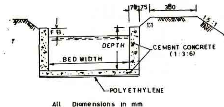
Fig. 22 Typical Cement Concrete Section
