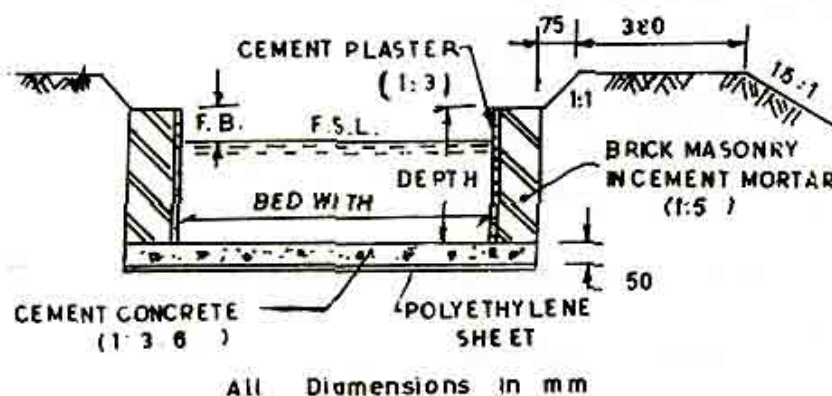
Fig. 21 Typical Cement Concrete And Brick Masonry Section
