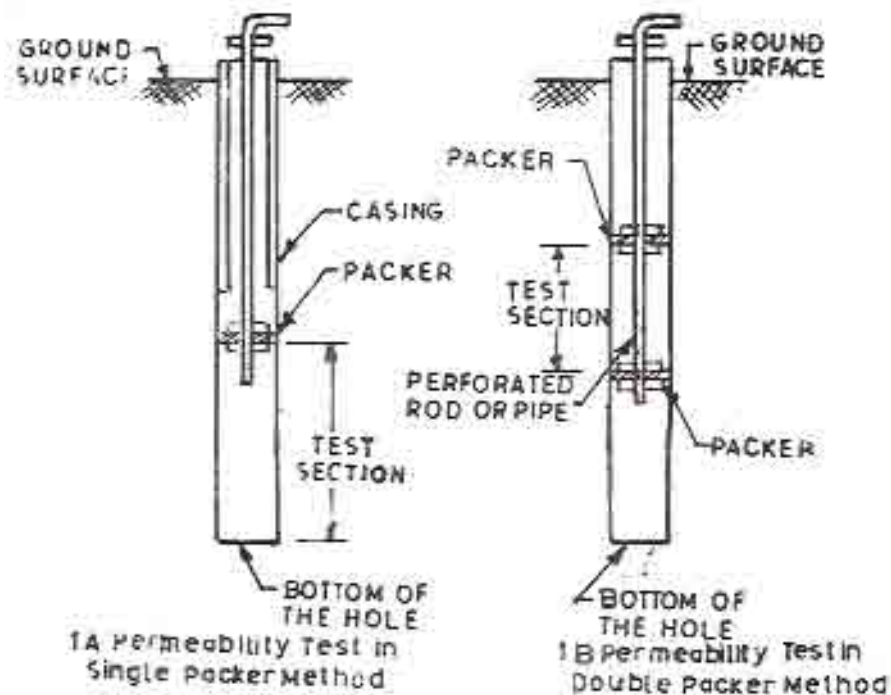
Fig 1. Permeability Test Both in Single and Double Packer Method
