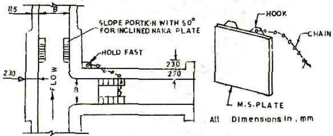
Fig. 24 Typical Design Of M.S. Plate Nakka Structure
