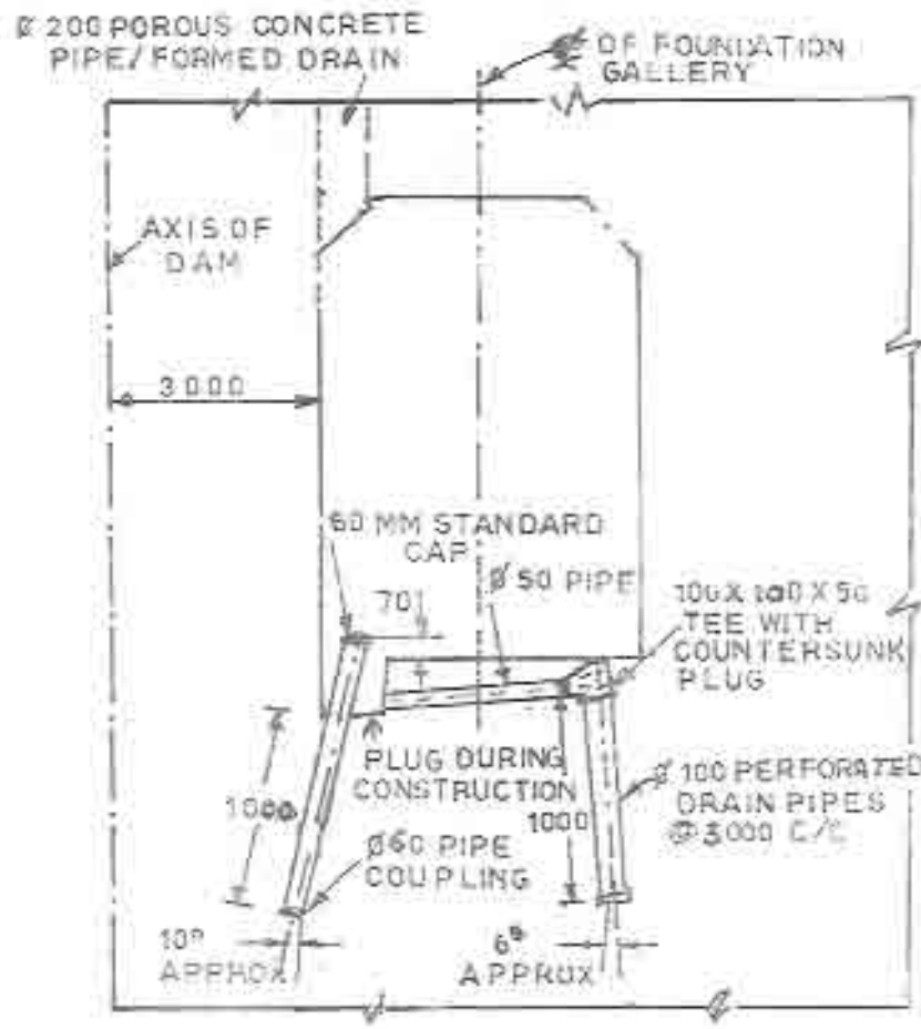
Fig. 5. Uplift Gauge
