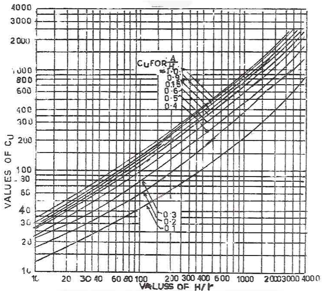
Fig. 10 CONDUCTIVITY COEFFICIENT FOR PERMEABILITY DETERMINATION IN UNSATURATED STRATA WITH PARTLY PENETRATING CYLINDRICAL TEST WELLS
