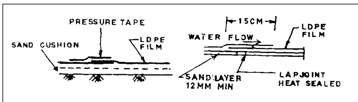
FIG. 11 (v) OVERLAP JOINT WITH PRESSURE TAPE
