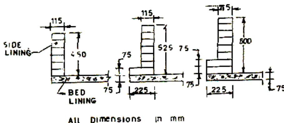
Fig. 20 Typical Section Of Side Walls
