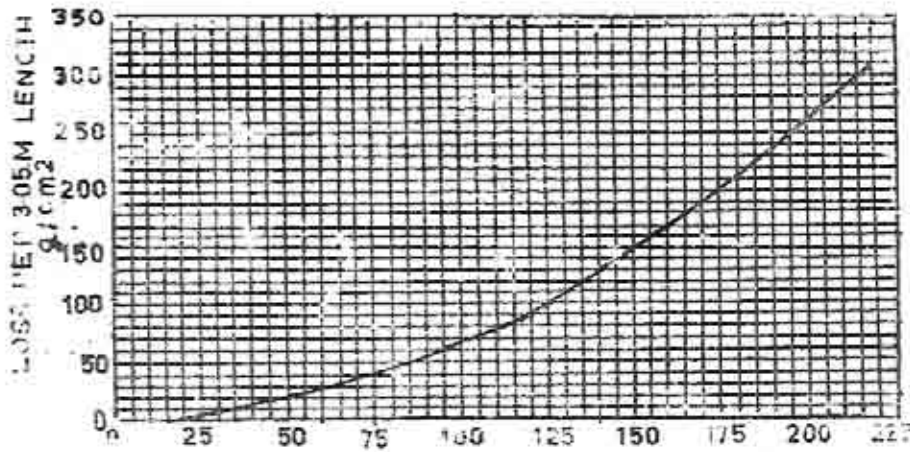
8C : HEAD LOSS PER 3.05 M SECTION OF BX DRILL ROD
