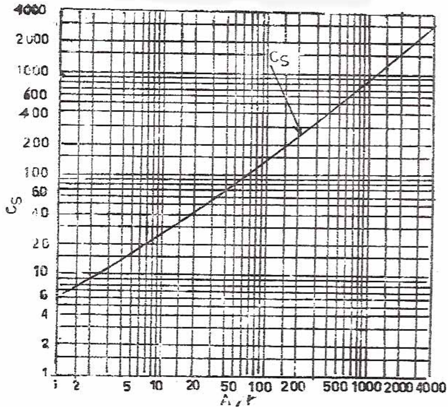
FIG. 11 : CONDUCTIVITY COEFFICIENTS FOR SEMI-SPHERICAL FLOW IN SATURATED STRATA THROUGH PATIALLY PENETRATING CYLINDRICAL TEST WELLS
