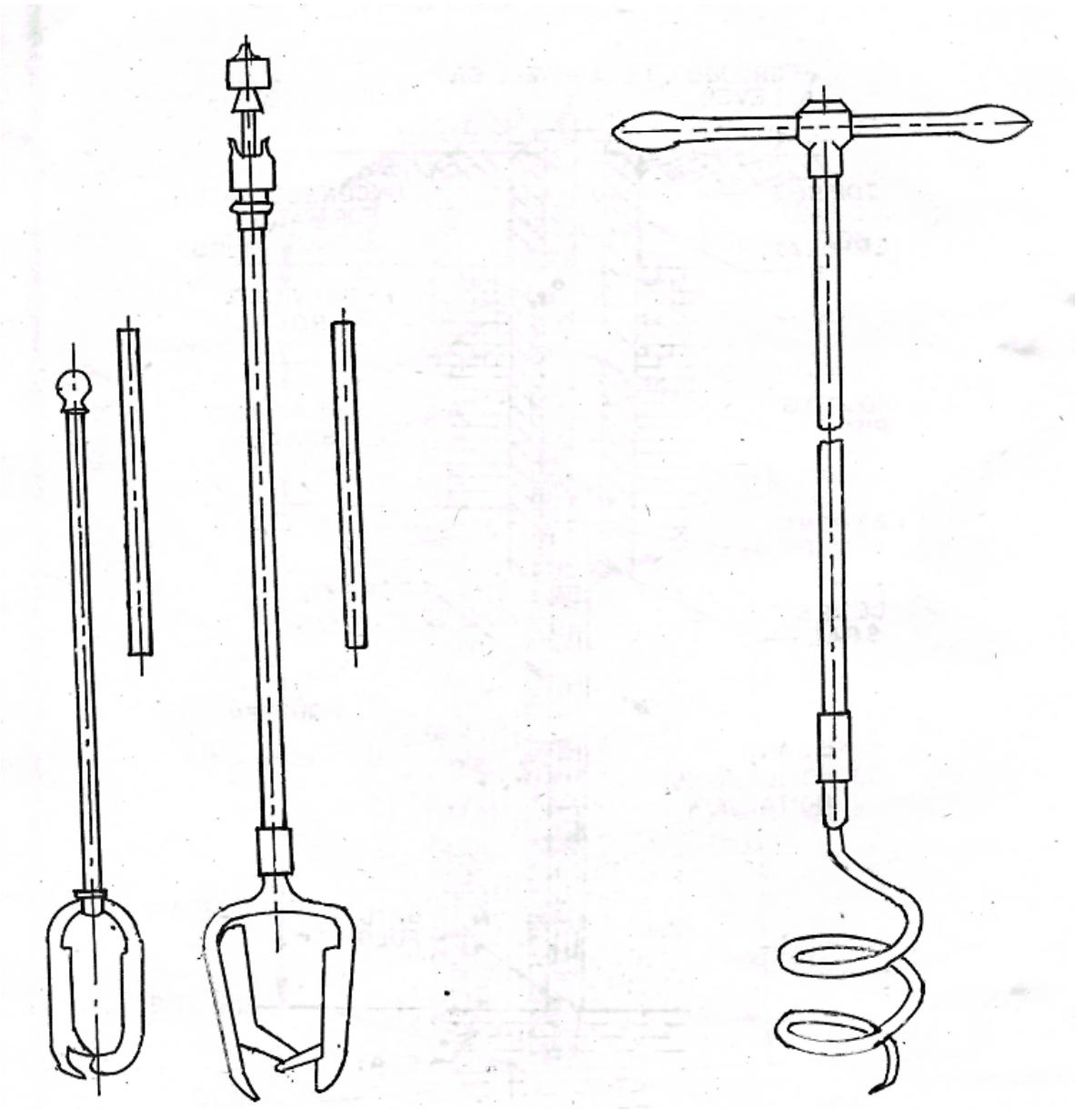
B. SPIRAL AUGER OR RAM'S HORN
