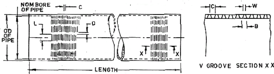
FIG 'A'- BRASS SCREENS WITH VERTICAL SLOTS
