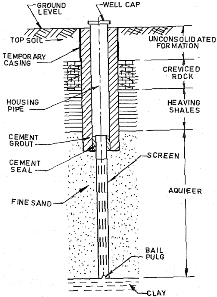
SLOTTED TUBEWELL (CREVICED FORMATION)
