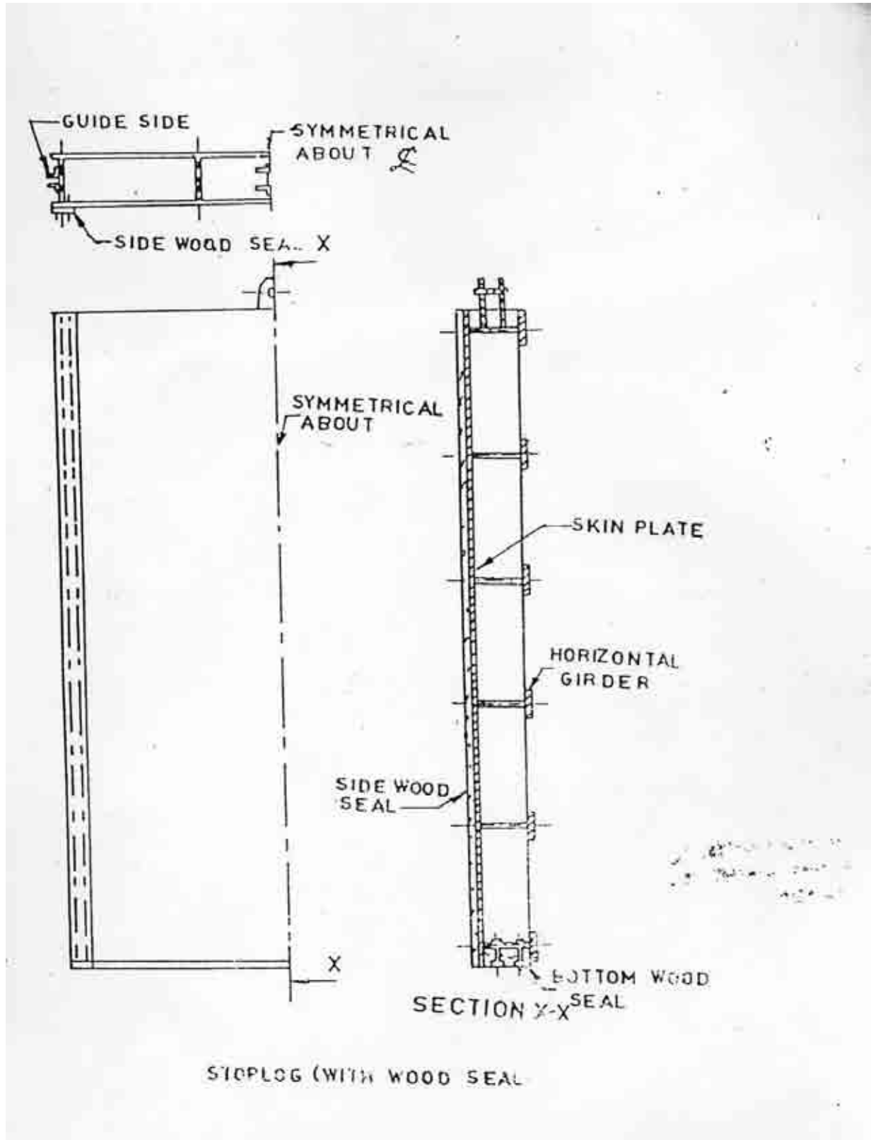
FIG. 2E. LOW HEAD SLIDE GATE SEALING AND ARRANGEMENT
