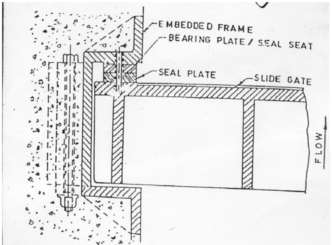
TYPICAL SLOT SECTION DETAIL SHOWING LOW HEAD SLIDE GATE AND EMBEDDED FRAME
