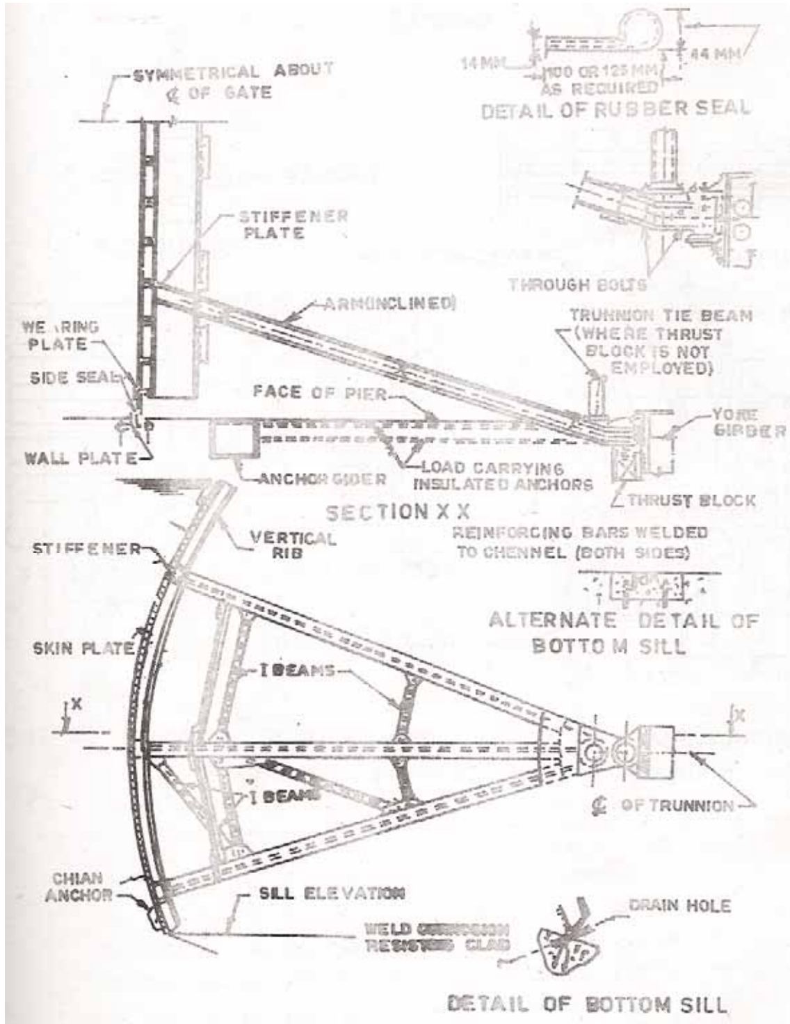
FIG. 3B. RADIAL GATE WITH INCLINED ARM
