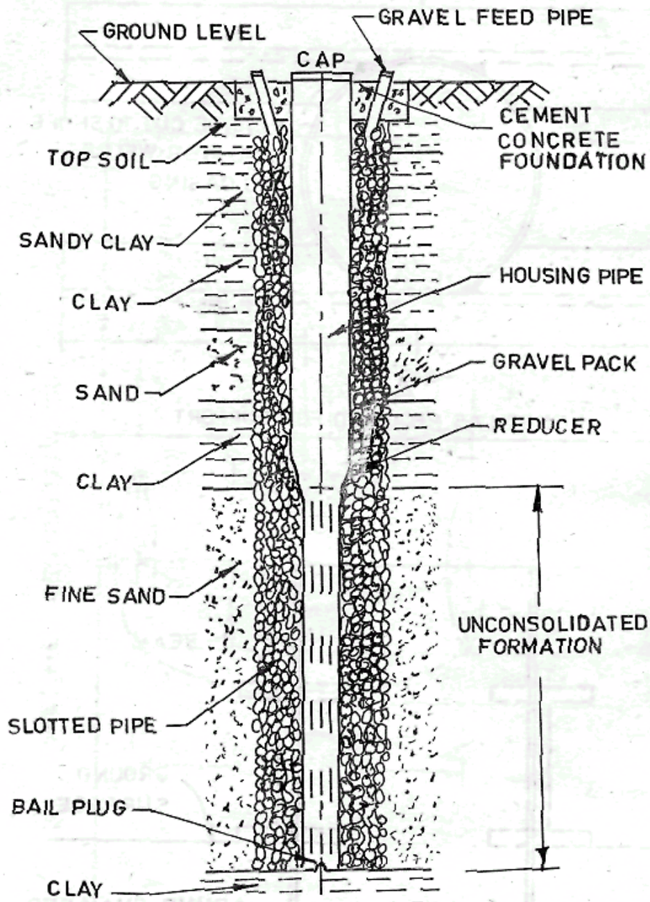
SLOTTED WELL (ARTIFICIAL GRAVEL PACK)
