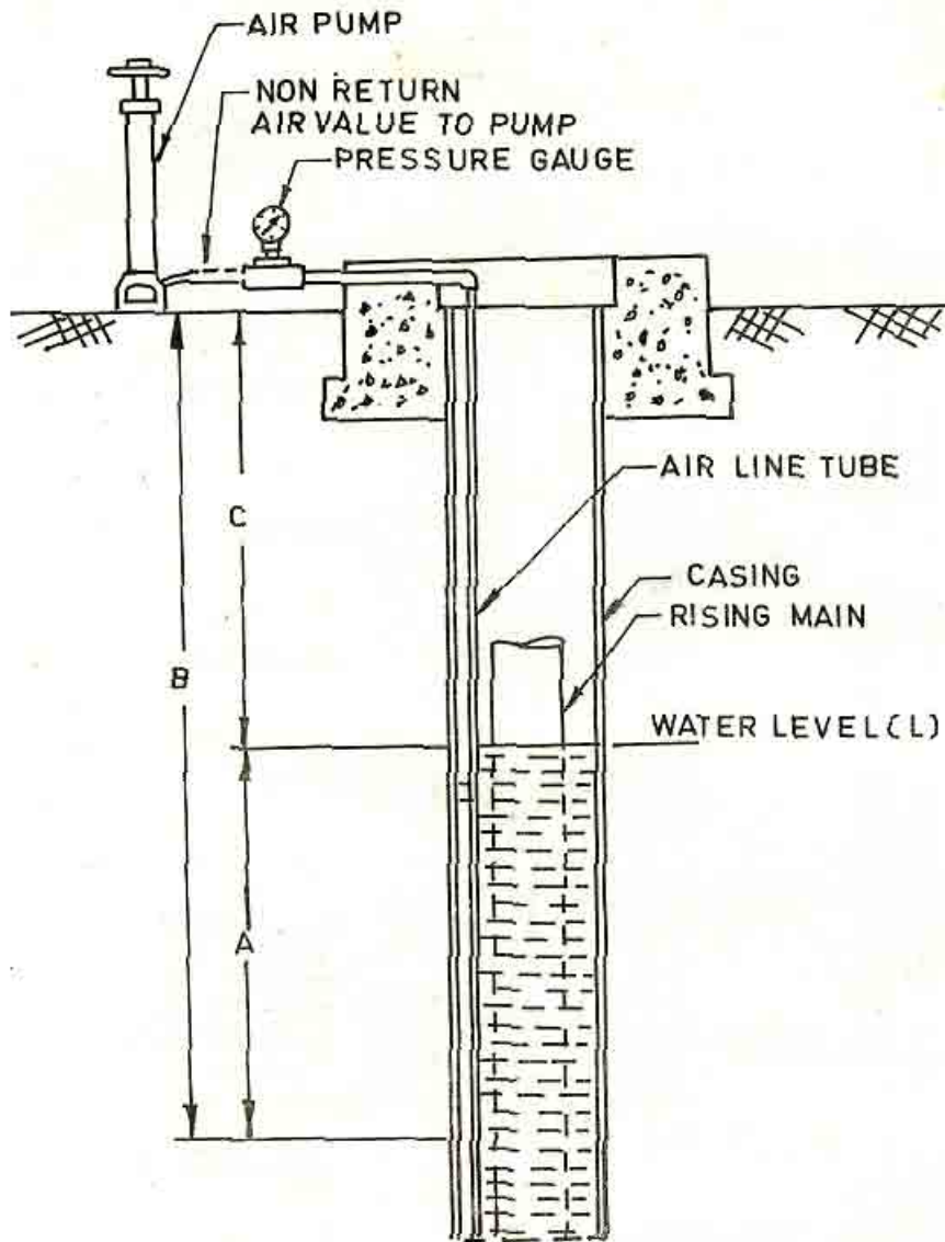
AIR PRESSURE LINE APPARATUS FOR DETERMINING THE WATER LEVEL IN A TUBEWELL
