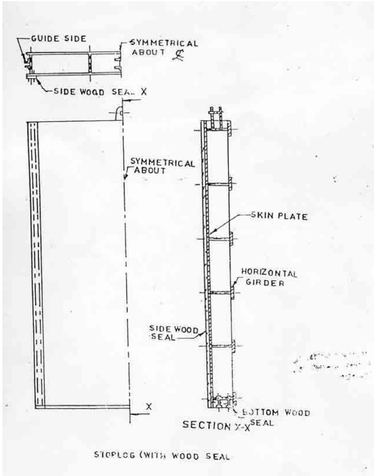
FIG. 2F. LOW HEAD SLIDE GATE SEALING ARRANGEMENT
