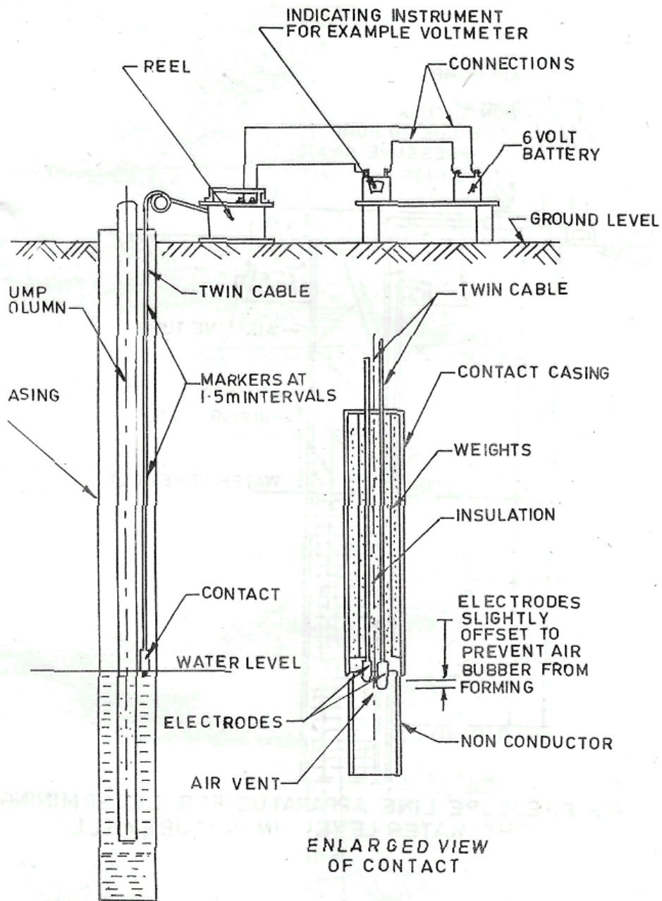
ELECTRICAL APPARATUS WITH DOUBLE POLE CONTACT FOR DETERMINING THE WATER LEVEL IN A TUBEWELL
