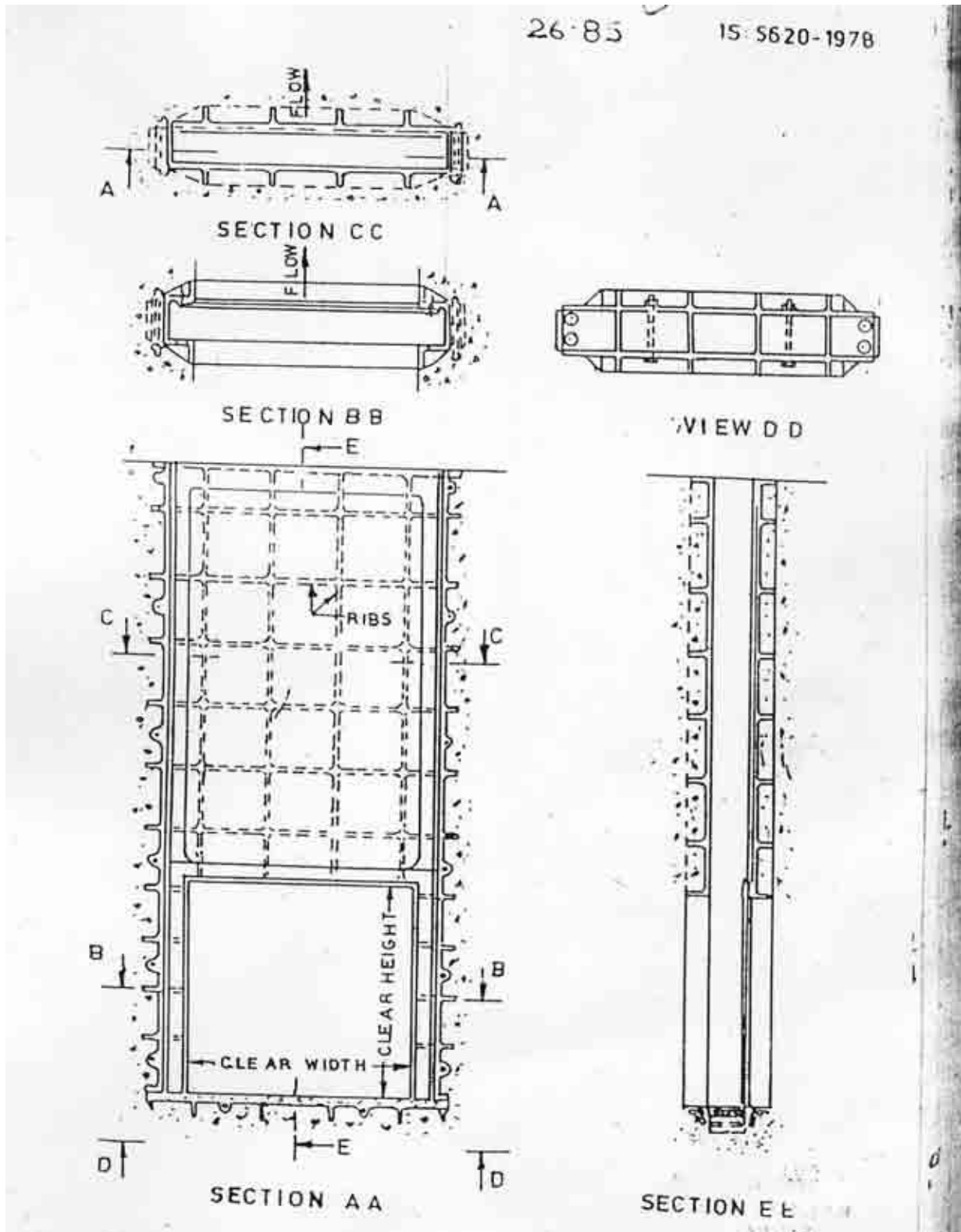
FIG. 2C. TYPICAL DIAGRAM SHOWING EMBEDDED FRAME OF LOW HEAD SLIDE GATE
