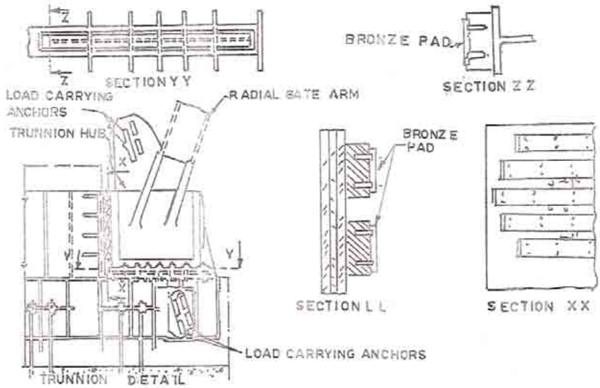
FIG. 3C. ARRANGEMENT FOR ALLOWING AND ELONGATION OF THE INSULATED LOAD CARRYING ANCHORS
