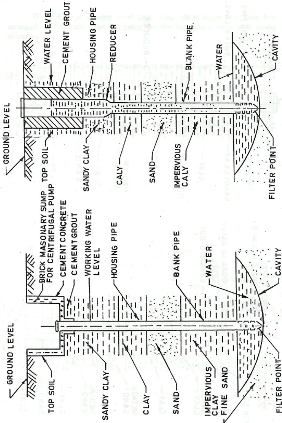
CAVITY WELL FOR TURBOMERSIBLE PUMP
