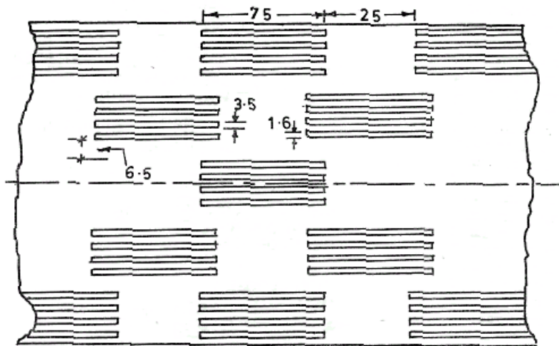
FIG.2 SLOTTING ARRANGEMENT
