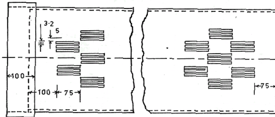
FIG.1 DEVELOPED VIEW OF A TYPICAL WELL SCREEN PLAIN, SLOTTED TYPE
