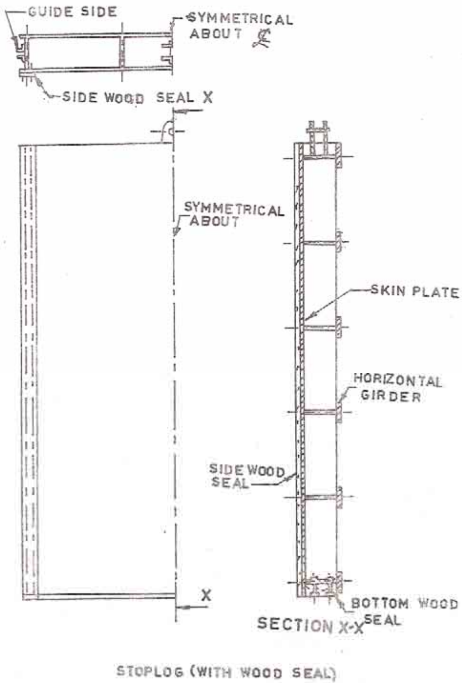
FIG 2F LOW HEAD SLIDE GATE SEALING ARRANGEMENT
