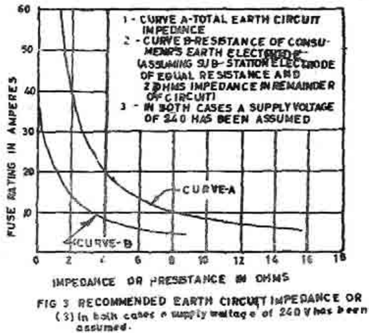
Fig. 3 Recommended Earth Circuit Impedance
