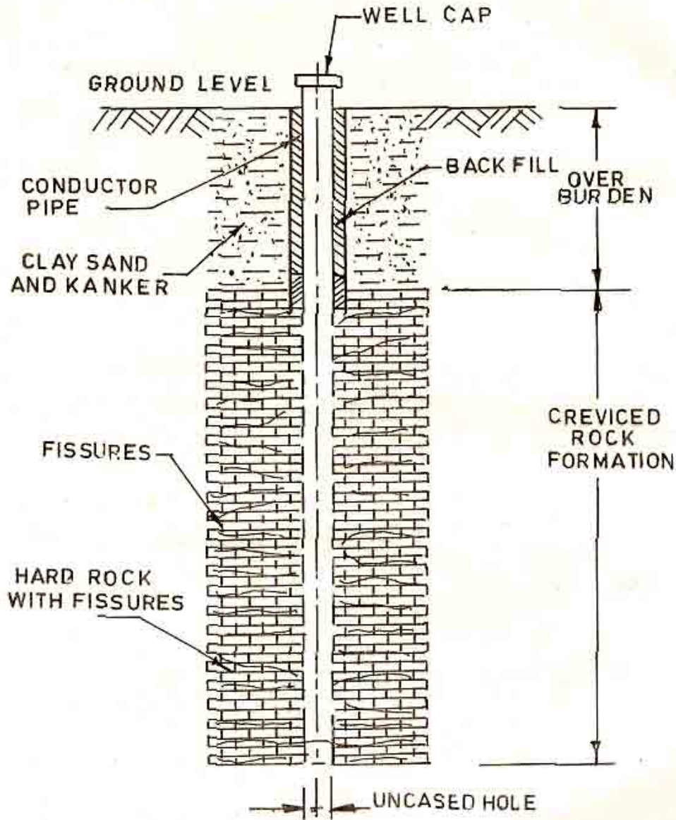
TUBEWELL IN HARD ROCK
