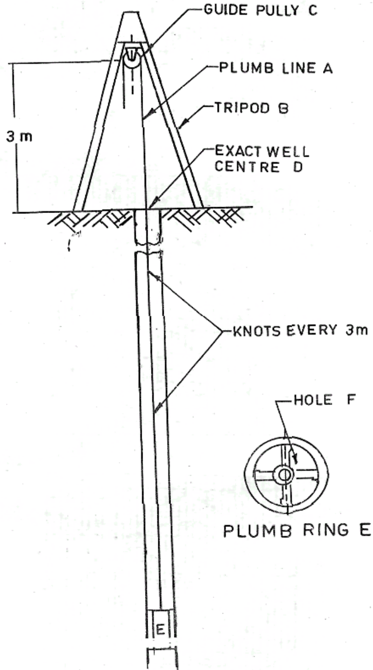
METHOD OF PLUMBING A WELL
