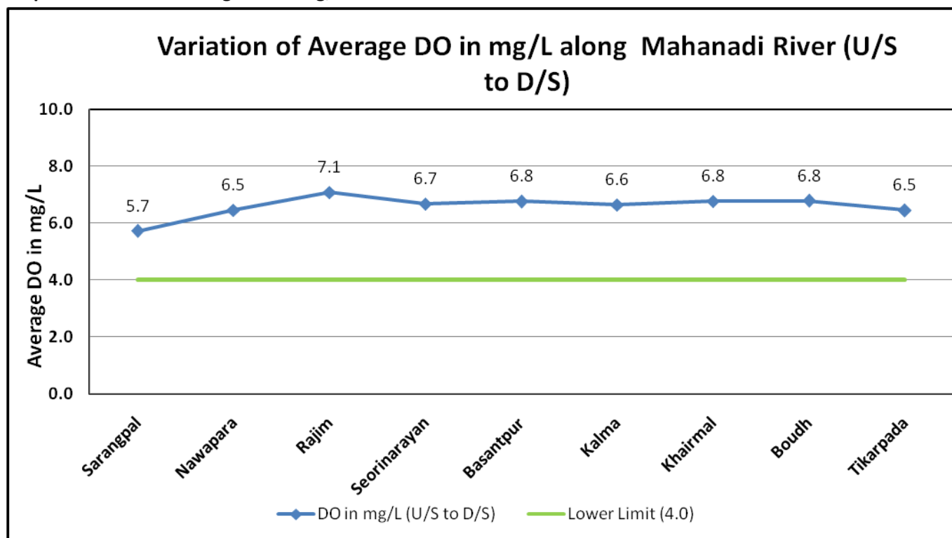
Graph: Variation of Average DO in mg/L
