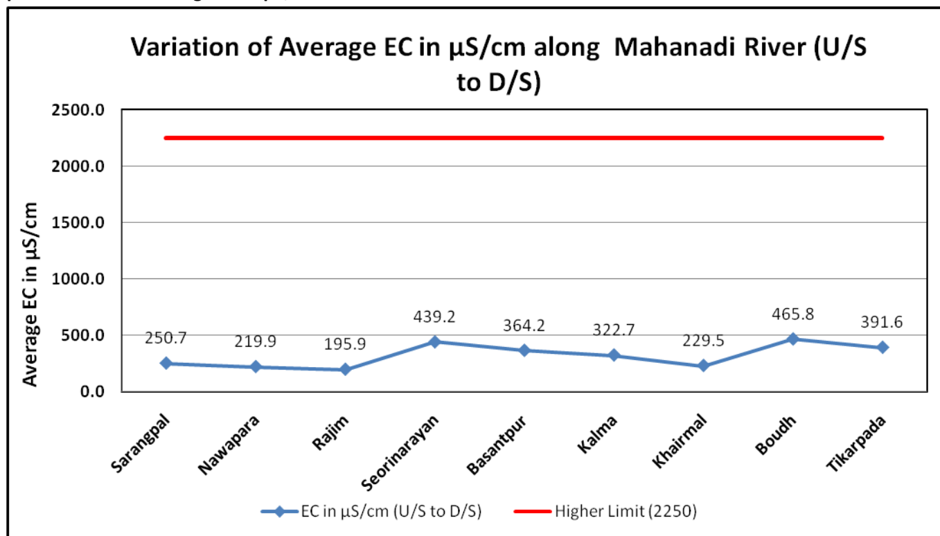
Graph: Variation of Average EC in \mu\text{S/cm}
