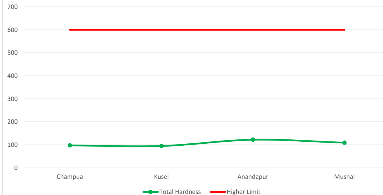
Variation of Total Hardness from U/S to D/S along Baitarani Basin
