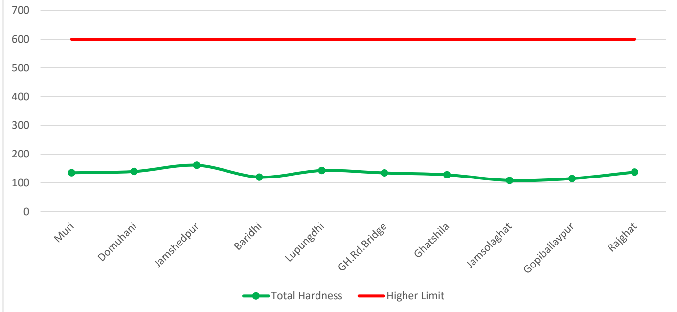
Variation of Total Hardness from U/S to D/S along Subarnarekha River
