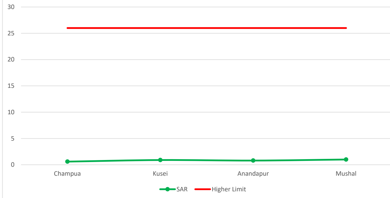
Variation of Sodium Adsorption Ratio from U/S to D/S along Baitarani Basin
