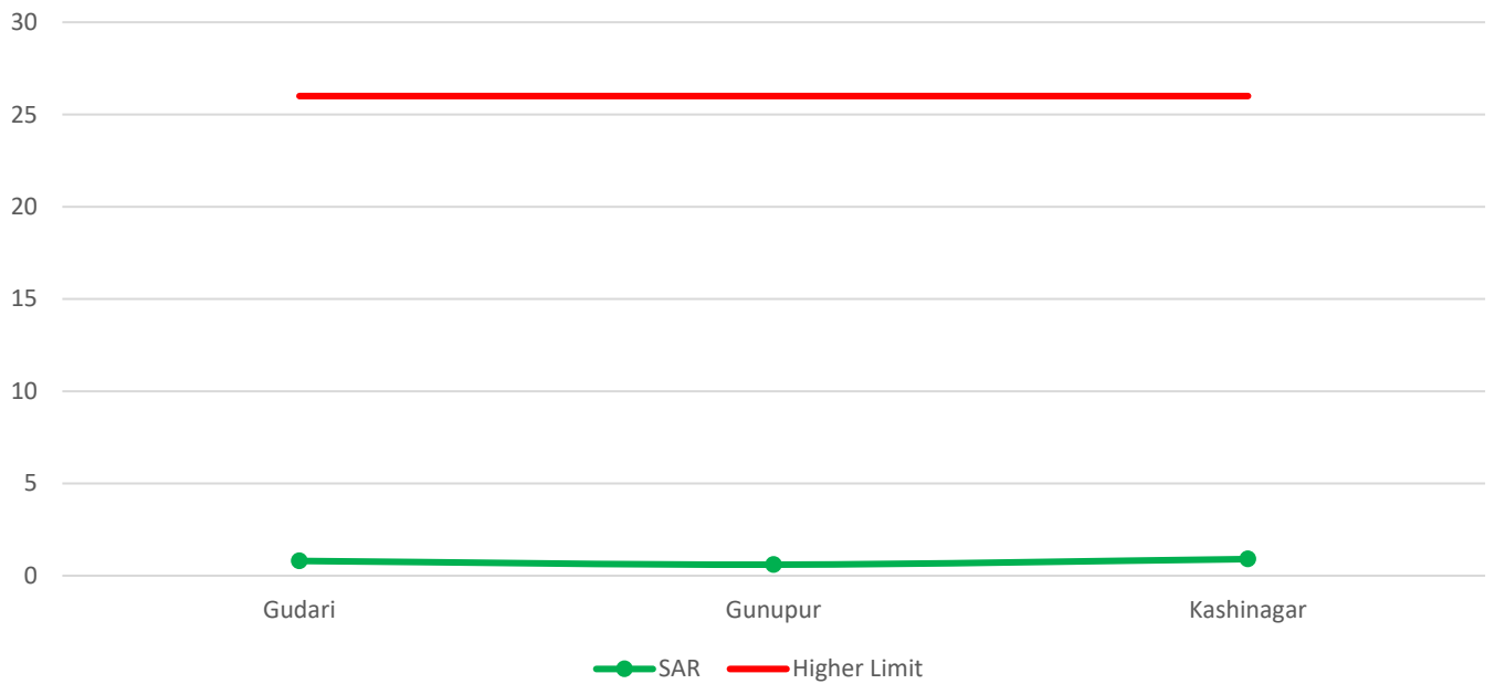
Variation of Sodium Adsorption Ratio from U/S to D/S along Vamsadhara River
