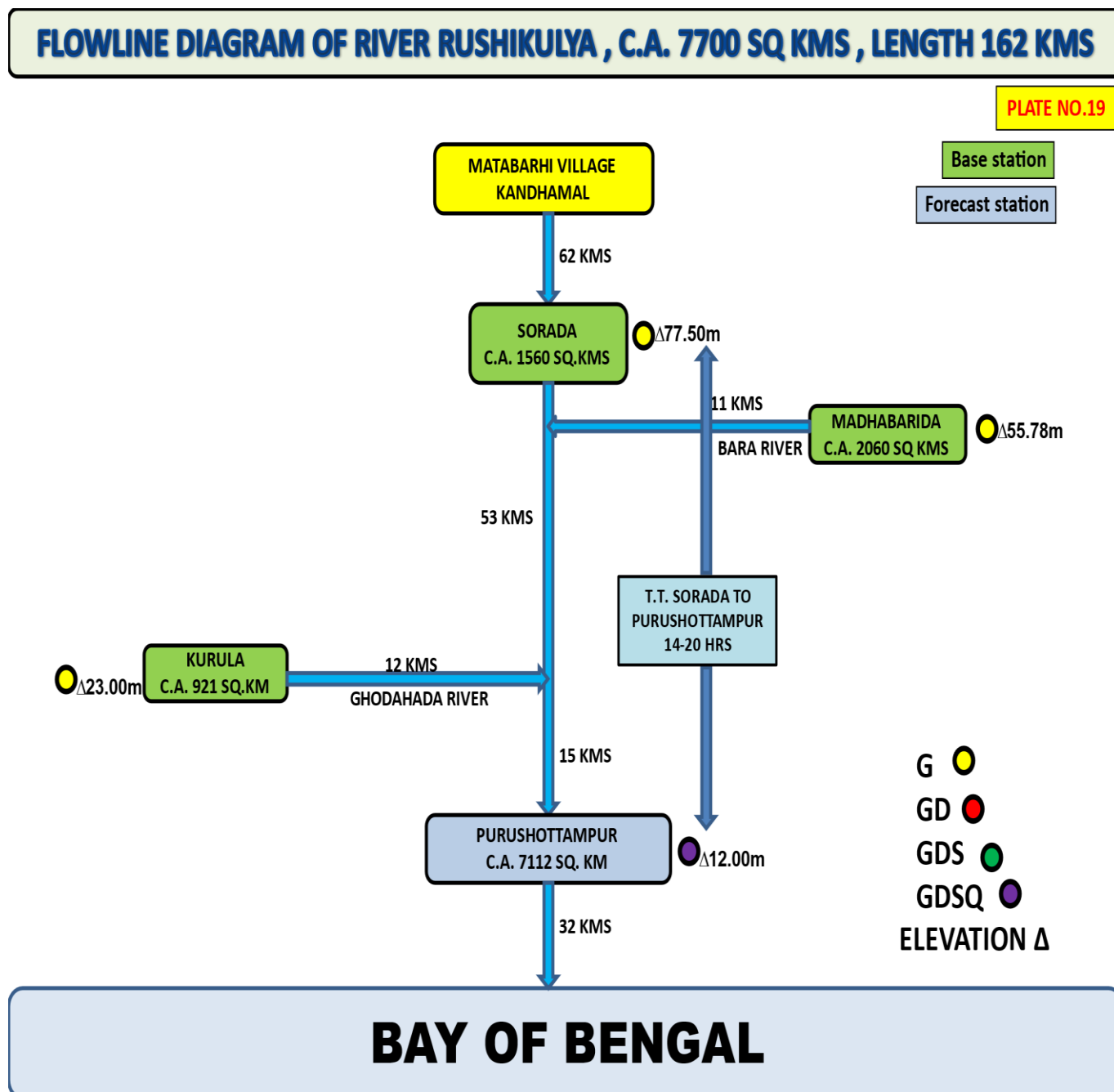
Fig- 8.0 (The flow line diagram of Rushikulya River)
