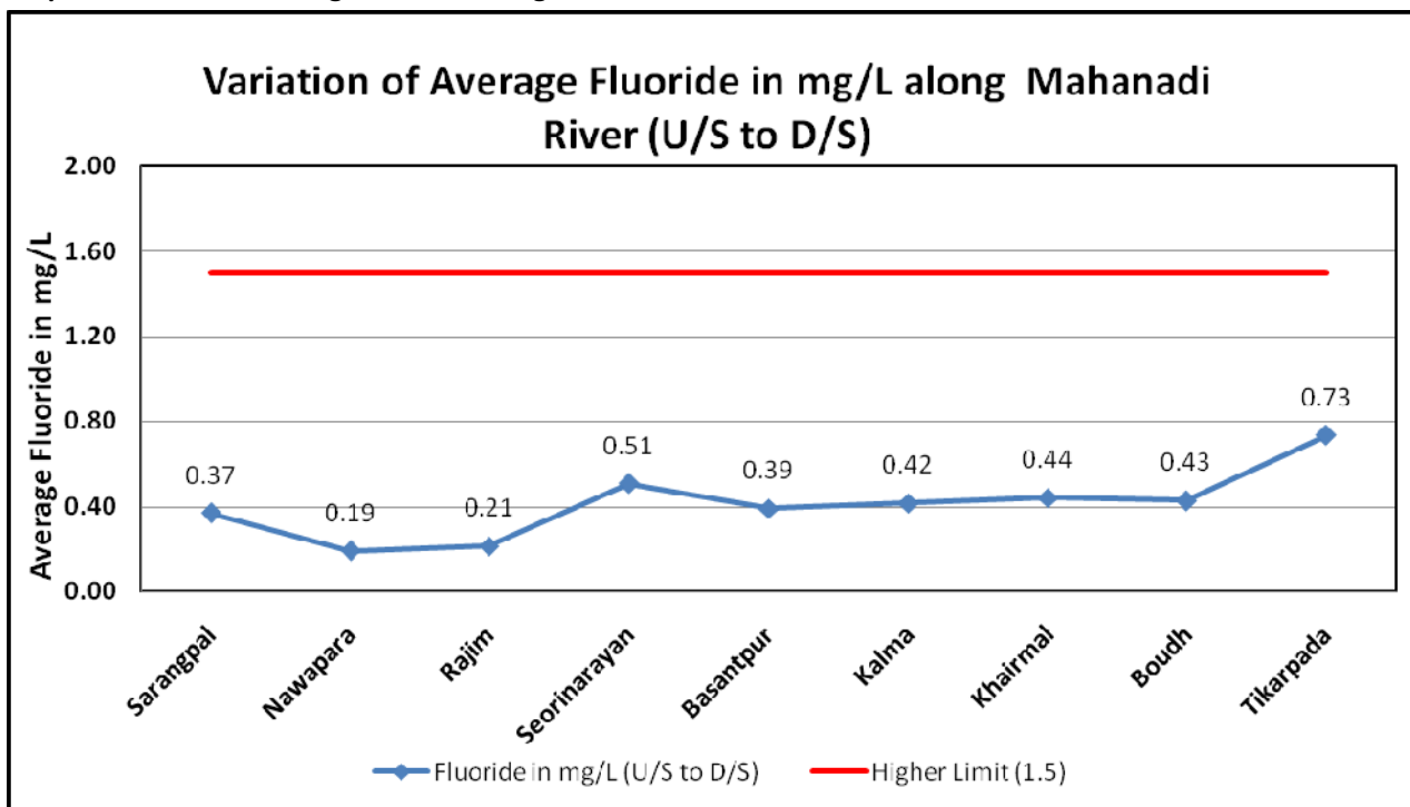
Graph: Variation of Average Fluoride in mg/L.
