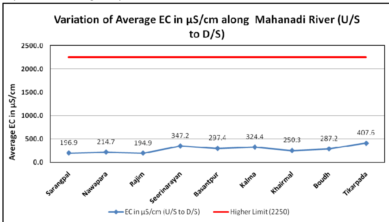
Graph: Variation of Average EC in \mu\text{S/cm}
