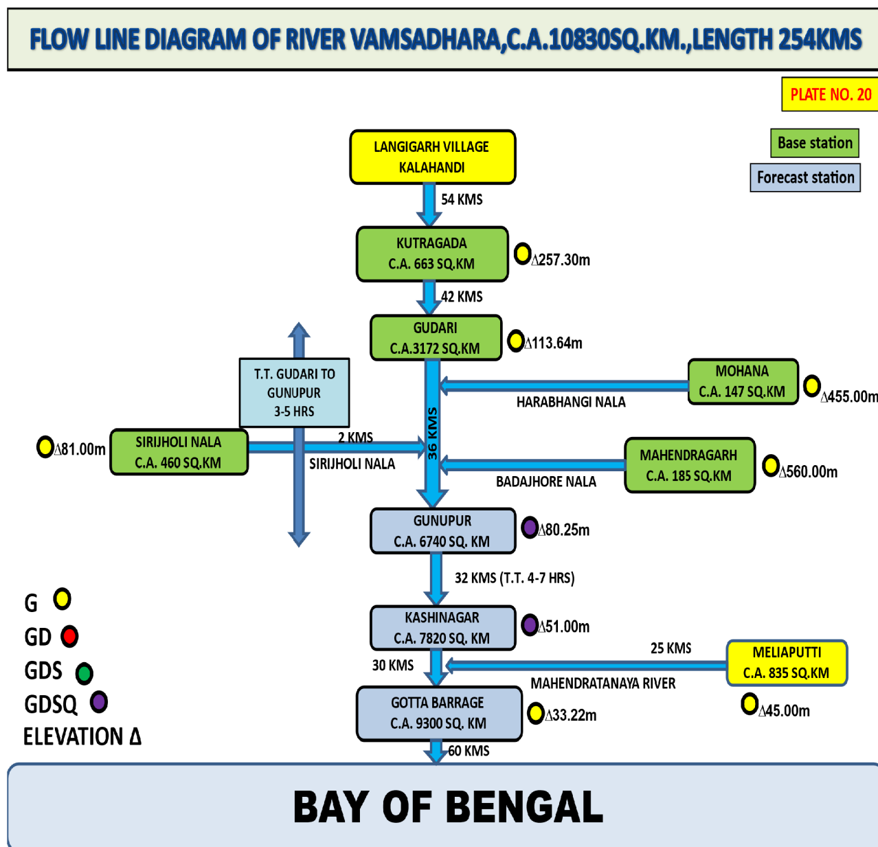
Fig-11.0 (Flowline diagram of the Vamsadhara River)
