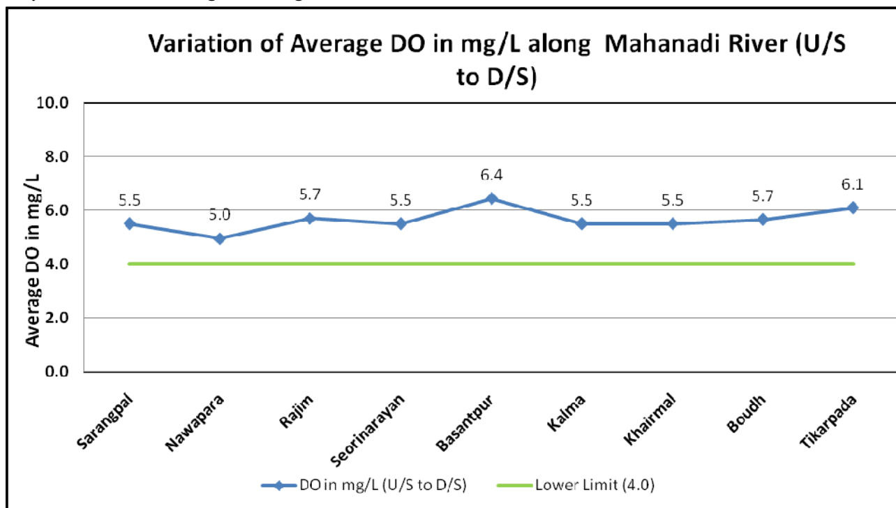
Graph: Variation of Average DO in mg/L
