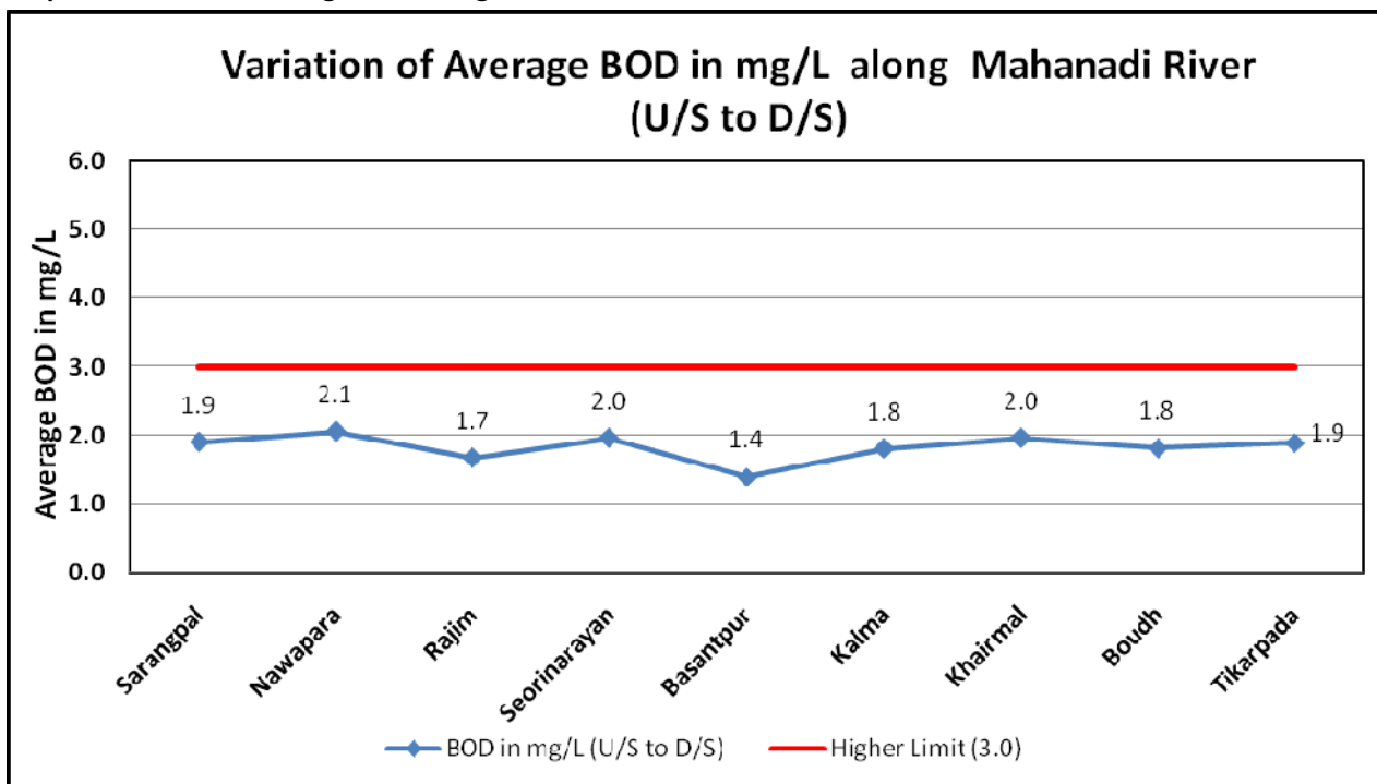
Graph: Variation of Average BOD in mg/L
